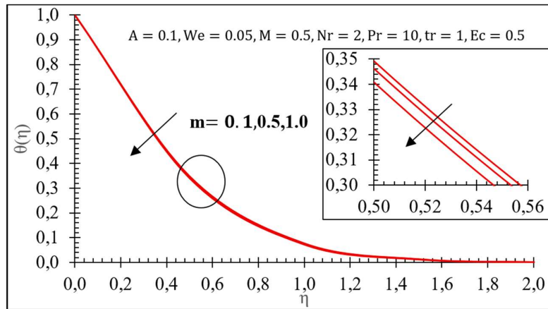
Fig.7. Variation in temperature behaviour \theta(\eta) .
