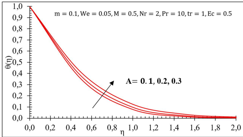
Fig.10. Variation in temperature behaviour \theta(\eta) .
