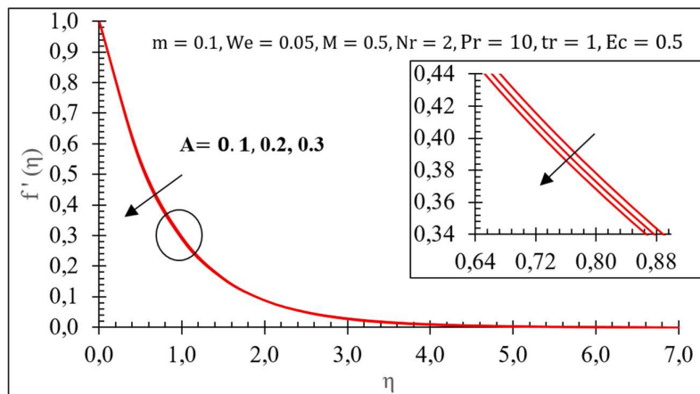
Fig.8. Variation in f''(\eta) .
