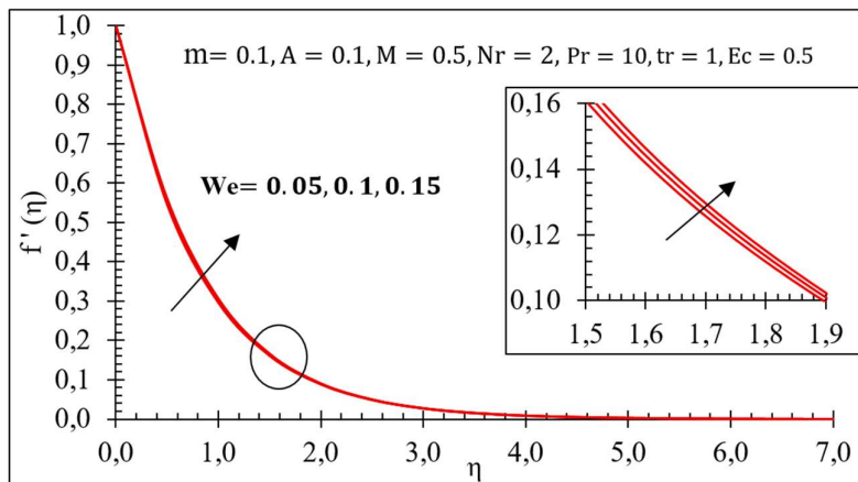
Fig.11. Variation in f''(\eta) .
