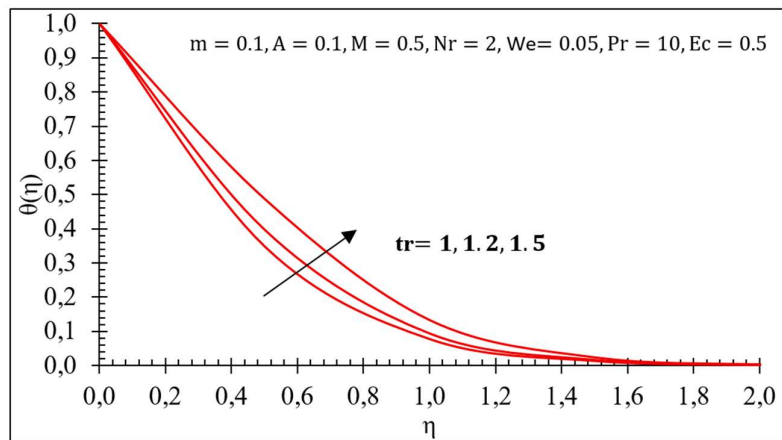
Fig.16. Variation in temperature behaviour \theta(\eta) .
