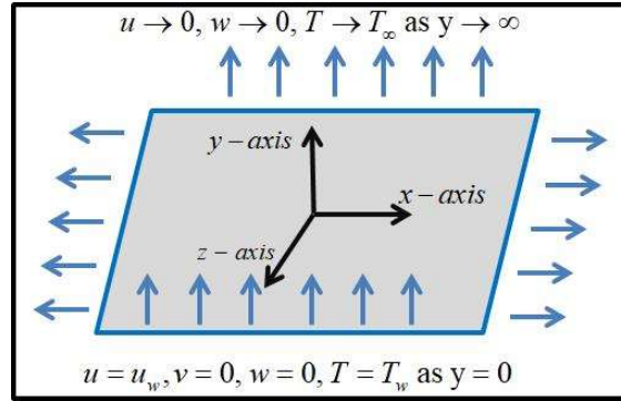
Fig.1. Configuration of the flow.
