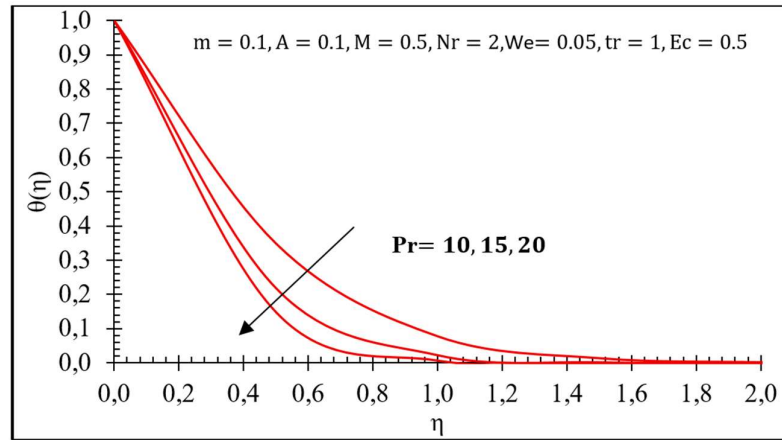
Fig.15. Variation in temperature behaviour \theta(\eta) .
