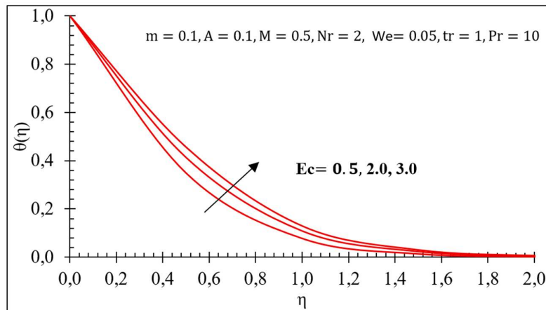
Fig.17. Variation in temperature behaviour \theta(\eta) .
