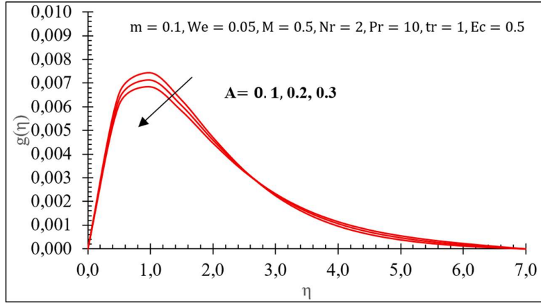
Fig.9. Variation in g(\eta) .
