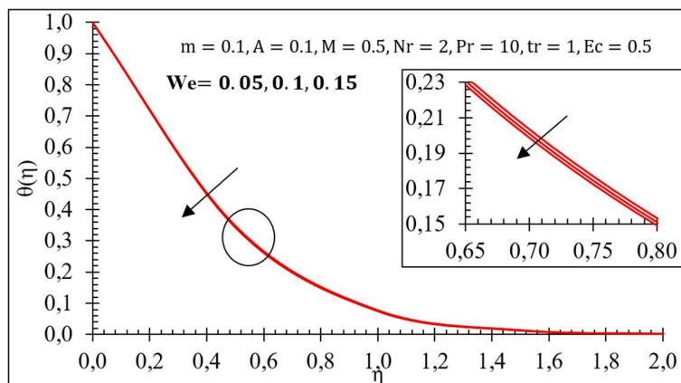
Fig.13. Variation in temperature behaviour \theta(\eta) .
