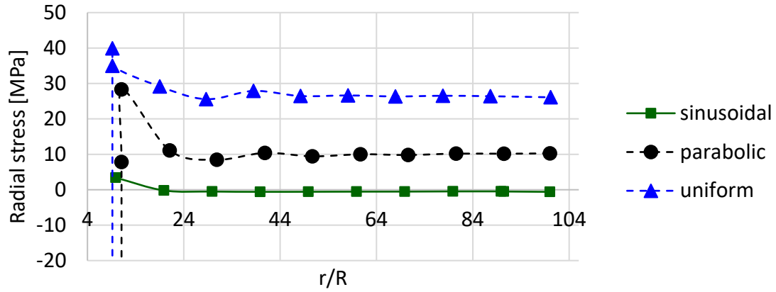
Fig.9. Normalised radial stress components for uniform, sinusoidal, and parabolic distributions along the vertical radius.
