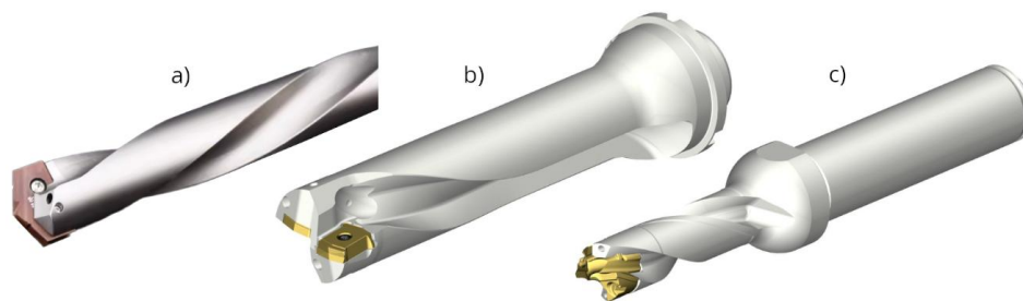
Fig.14. Drills with indexable inserts: a) drill with an exchangeable blade [22], b) indexable insert drill [23], c) drill with an exchangeable head [23].
