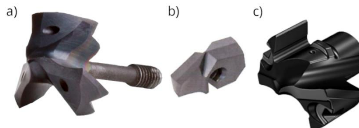
Fig.15. Exchangeable drill heads: a) with a threaded shank [24], b) exchangeable blade [22], c) clamped head [23].
