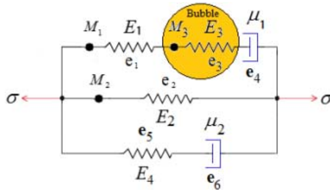
Fig.2. Three-branch rheological scheme including a gas bubble.
